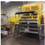
Uniloy Model 350 R3 (6) Head Blow Molding Machine
